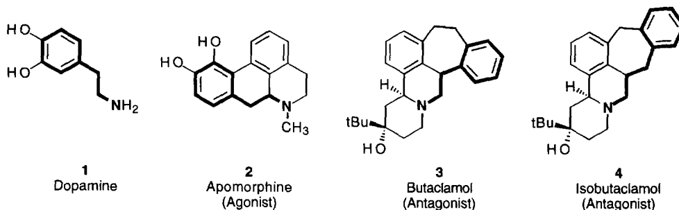
Figure 1. Some common dopamine analogs with the probable pharmacophore emboldened.
