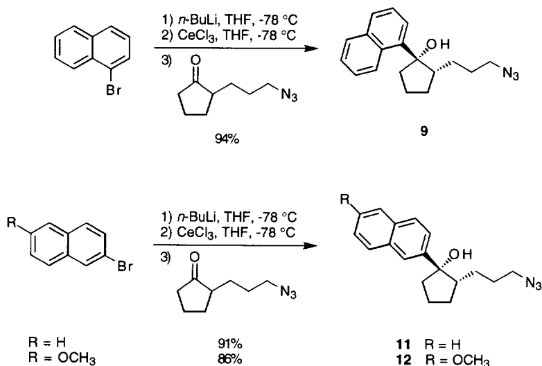
Scheme 3. Synthesis of the azido alcohols 9 , 11 , and 12 .
