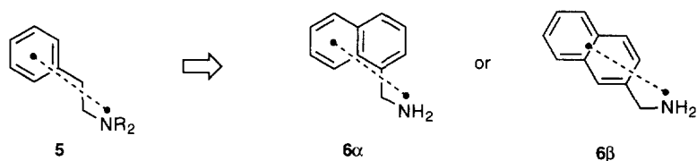
Figure 2. The distance \bullet ----- \bullet between the lone pair and the \pi -system of \beta -phenethylamine is also found in \alpha -naphthylmethylamine and \beta -naphthylmethylamine.
