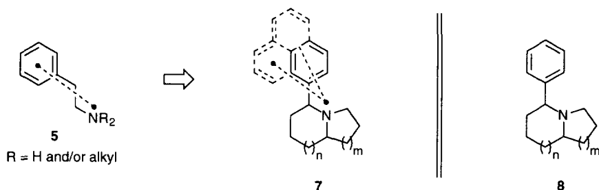
Figure 3. The \beta -phenethylamine mimics \alpha -naphthylamine and \beta -naphthylamine may be incorporated into a fused-bicyclic amine framework (i.e., 7 ). Similar aryl-substituted fused-bicyclic amines show antinociceptive activity, e.g. 8 . 19
