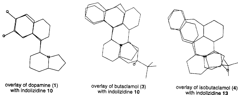
Figure 4. Structural comparisons 29 of indolizidine 10 with dopamine (1) and butaclamol (3), and indolizidine 13 with isobutaclamol (4).
