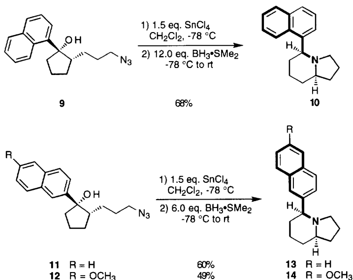
Scheme 2. Intramolecular Schmidt reactions produce the desired \alpha - and \beta -naphthylindolizidines.
