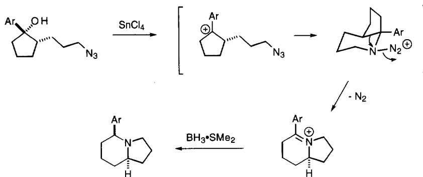
Scheme 1. The intramolecular Schmidt reaction may be used for the synthesis of 5-arylindolizidines.
